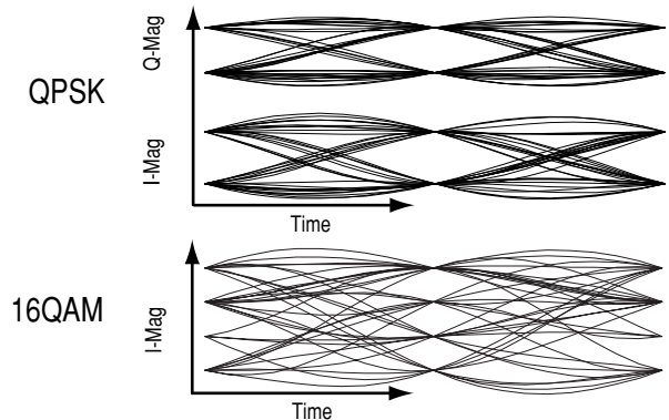
Figure 27. I and Q Eye Diagrams
